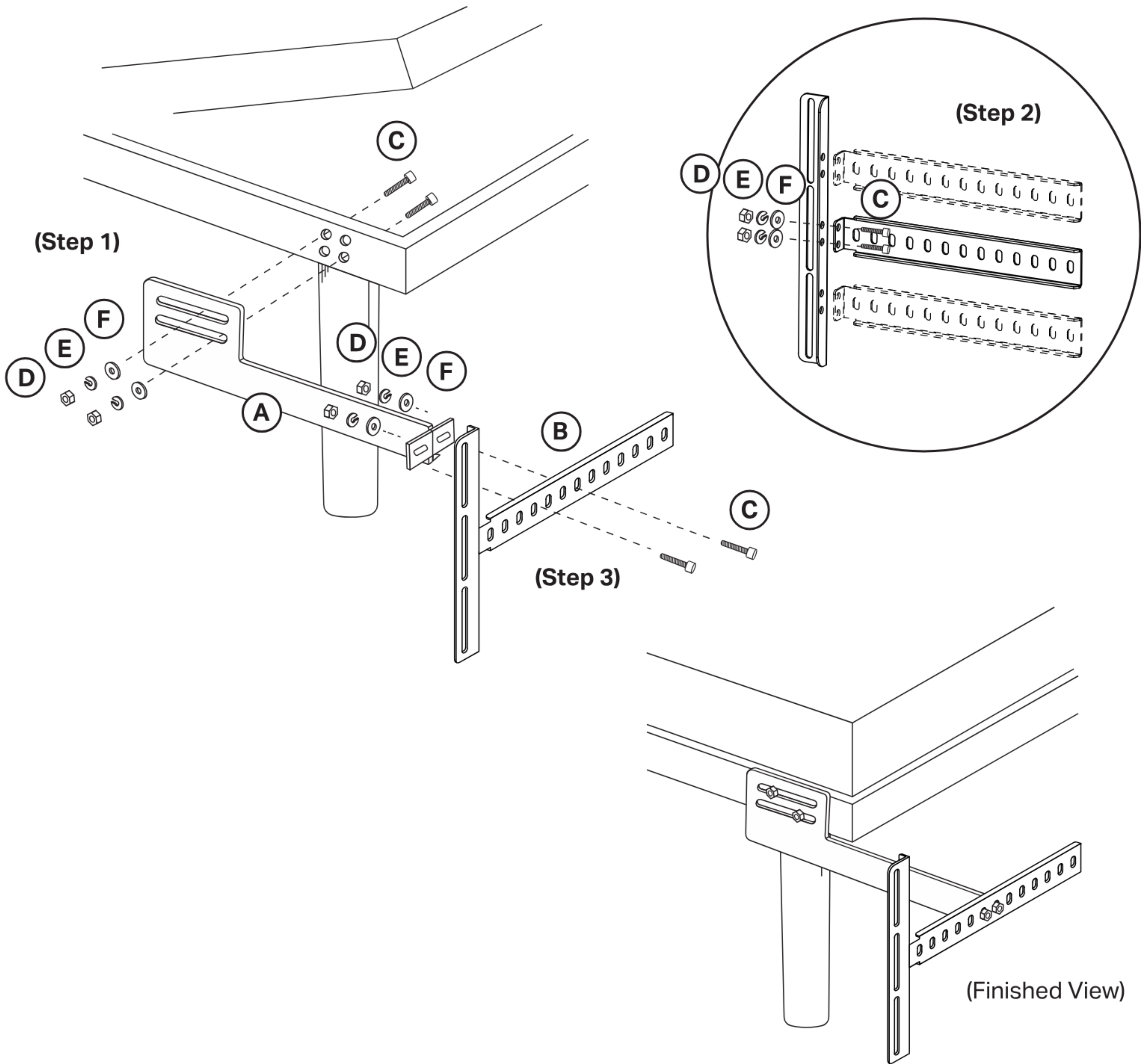
(2) Mounting Adapters
